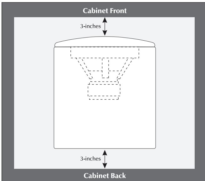
Figure 15. Placing the Abyss in a cabinet requires a minimum of three inches of open space on the front and back.
