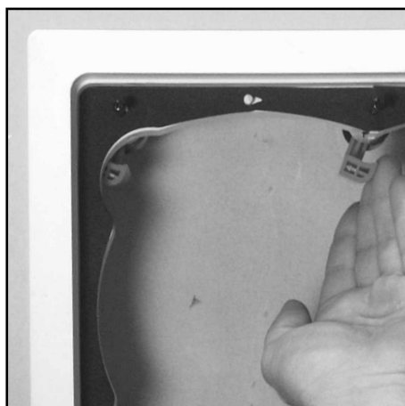
The swinging spring loaded dogs ease installation of the Mounting Kit/ Les brides à ressort d'oscillation soulagent l'installation du kit de support
